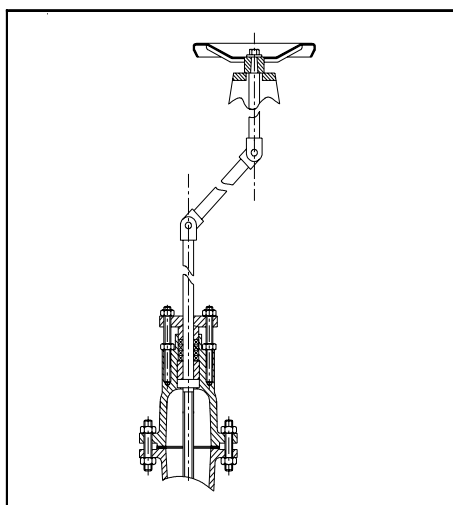
Var. 1050 Stem extension
