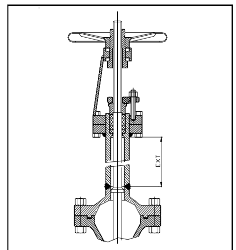
Var. 1060 Cryogenic extension
