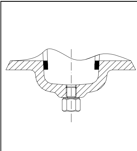
Var. 1200 Drain plug
