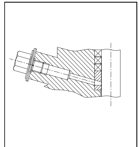
Var. 1030 Packing extraction system
