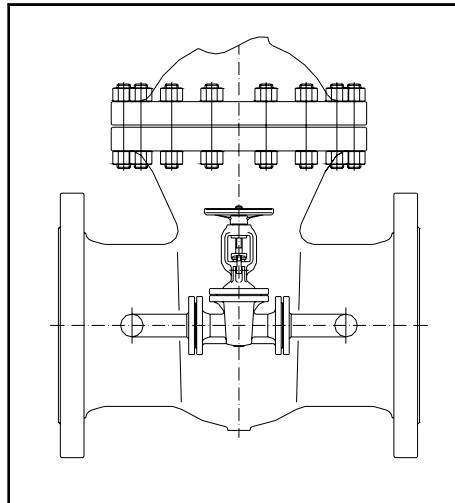
Var. 1300 By pass
