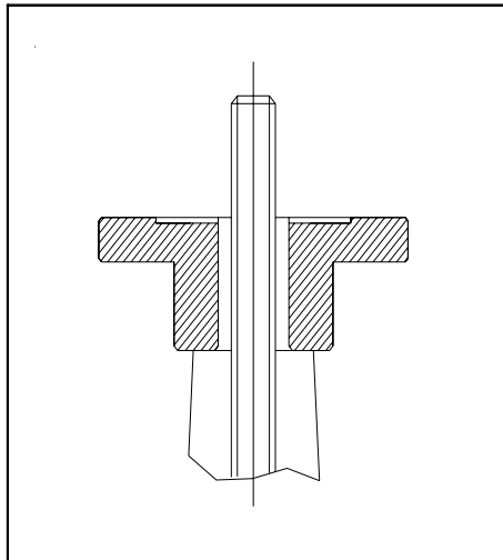
Var. 1010 Top flange acc. to ISO 5210
