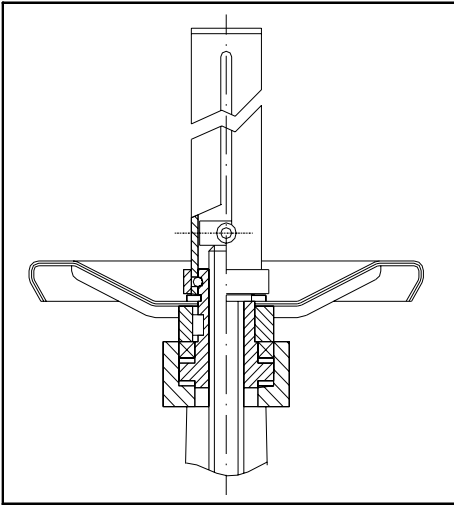
Var. 1110 Position indicator
