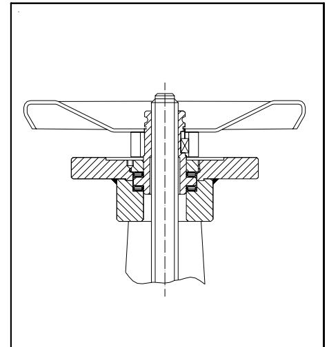
Var. 1015 Convertible top flange acc. to ISO 5210
