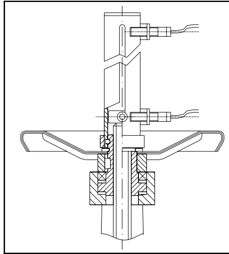
Var. 1120 Position indicator with limit switches
